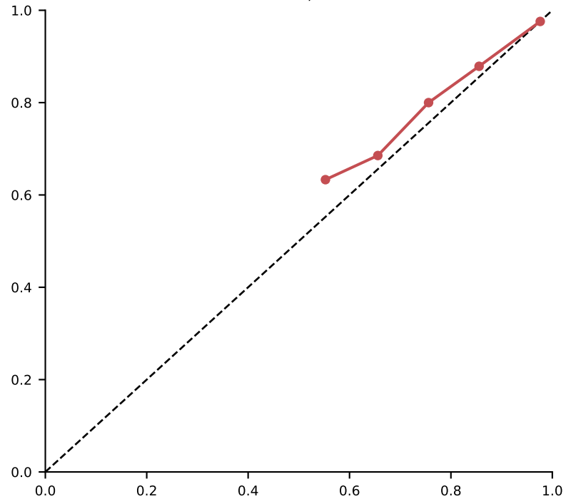
Unclustered ECE=0.008, n=4960
