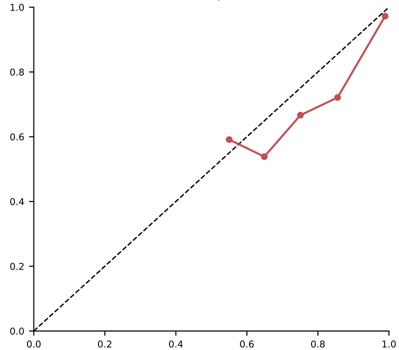
Clustered ECE=0.028, n=5413
